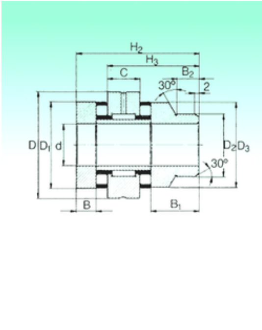
ZARN 65125 L TN Bearing 2D drawings and 3D CAD models
